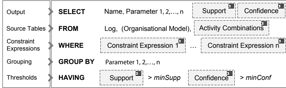
Fig. 2: SQL query assembly for querying declarative constraint templates
